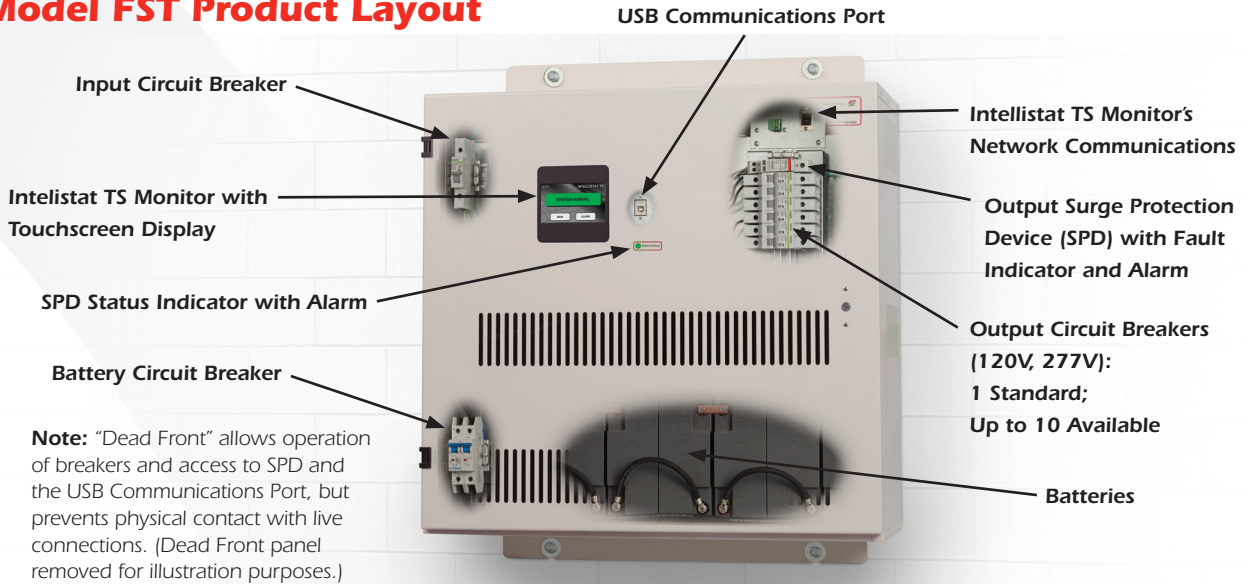
Wall-Mount Inverter shown with Intellistat TS Monitor
